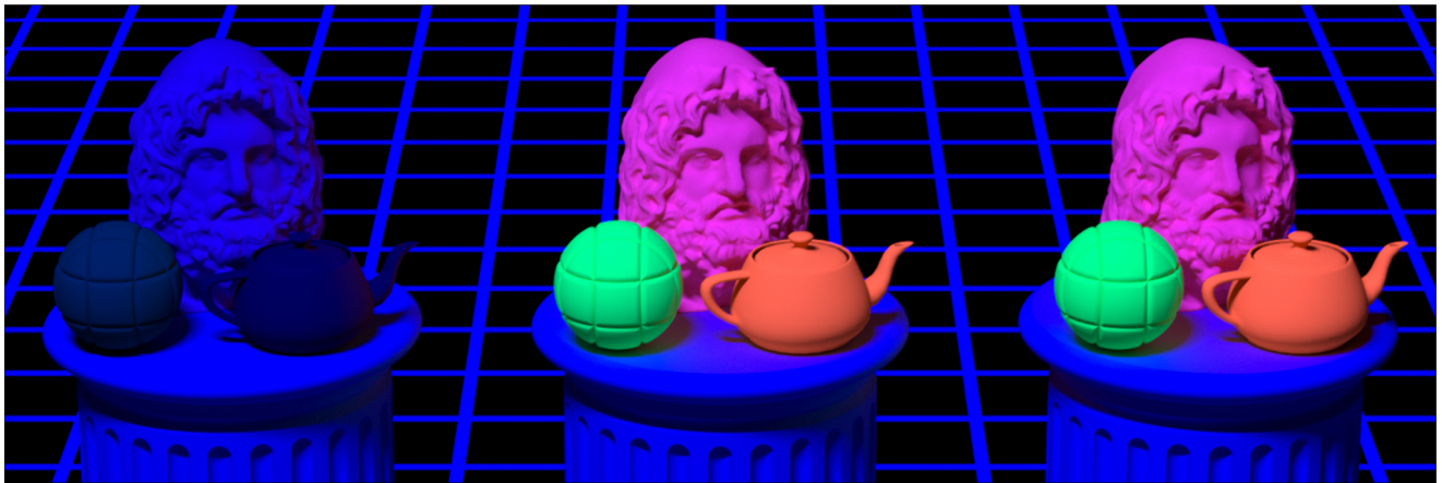
Figure 1: In this scene, we use a near-UV light for illumination. While non-fluorescent materials only reflect shades of the illumination colour (left), fluorescent surfaces also re-emit a portion of the absorbed energy from incident light as a light at additional wavelengths, leading to the colourful appearance of other objects in the scene. To represent fluorescent materials in a renderer, we typically use re-radiation matrices (centre), which have a significant memory overhead. Instead, we propose a more efficient representation of these matrices using Gaussian mixture models (right – eight Gaussians). Although compact, this representation also provides compelling results even with such challenging illumination.
