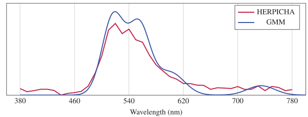
Figure 4: Comparison of conditional PDFs derived from a re-radiation matrix and its corresponding GMM representation. The figure shows the expected distribution of the re-emission wavelengths \lambda_o when the HERPICH A material is illuminated at \lambda_i = 440 nm. When a fluorescent event occurs, the outgoing wavelength \lambda_o is sampled according to this conditional PDF. Notice the presence of measurement noise lowering the highest values of the PDF derived from the raw re-radiation matrix after normalization compared to the PDF derived from the fitted GMM.
